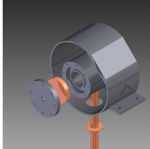
Figure 1: Schematic view of the cryogenic source
