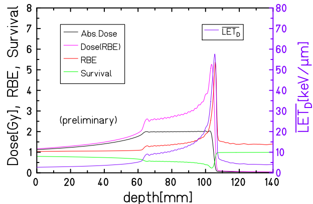
Figure 3: Depth profiles, including dose-mean LET.
