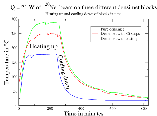
Figure 2: Preliminary results of test run with 20 Ne beam are shown. Heating and cooling responses of the pure densimet block are shown in green. The same is shown for the block with stainless steel welded strips and cerablack coating by the red and the blue solid lines, respectively. As seen in the picture, each densimet block was exposed to a beam (heating up) for about four hours. The decrease in temperature of each curve represents the cooling down of the corresponding block. For more details see text.
