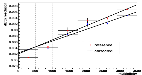
Figure 2: dE/dx resolution for different multiplicity bins.
