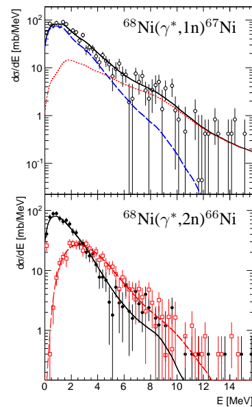
Figure 1: Neutron kinetic-energy differential cross sections. See text for description.
