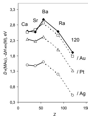
Fig. 1. Calculated D_e(\text{MAu}) (filled symbols) and -\Delta H_{\text{ads}}(M) (open symbols), where M = \text{Ca} through element 120, on Au, Pt and Ag.
