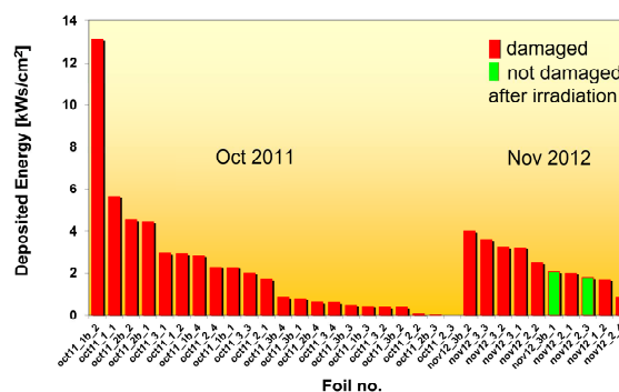
Fig. 3: Statistics of the irradiated foils (20 \mu\text{g}/\text{cm}^2 ).
