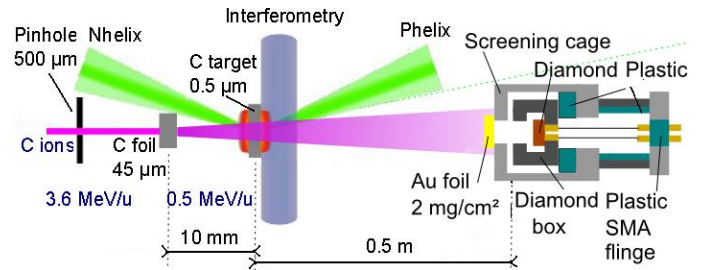
Figure 1: Experimental setup.
