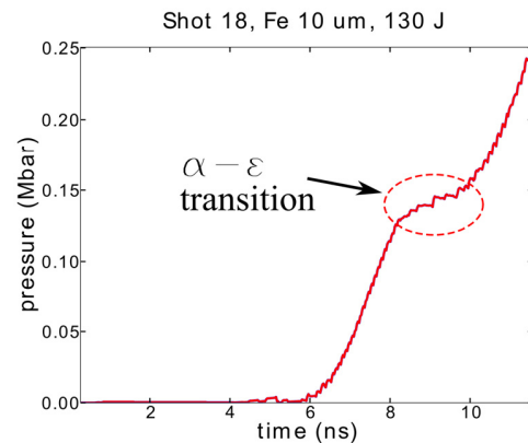
Figure 4: Pressure temporal profile with α-ε phase transition plateau.
