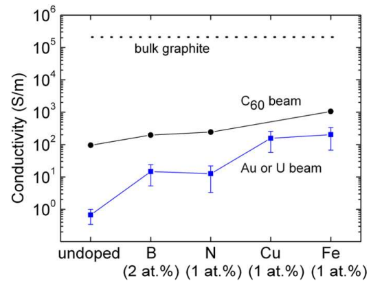
Figure 2: Conductivity of ion tracks for differently doped ta-C films. The beams were 1-GeV Au or U ions (for Cu) and 30-MeV C 60 clusters [3]. The conductivities were calculated assuming a cylinder of 8 nm diameter and a length corresponding to the film thickness (100 nm).
