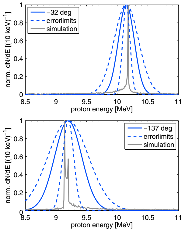
FIG. 6. The measured and simulated particle spectra for \Phi_s = -32 \text{ deg} and \Phi_s = -137 \text{ deg} .
