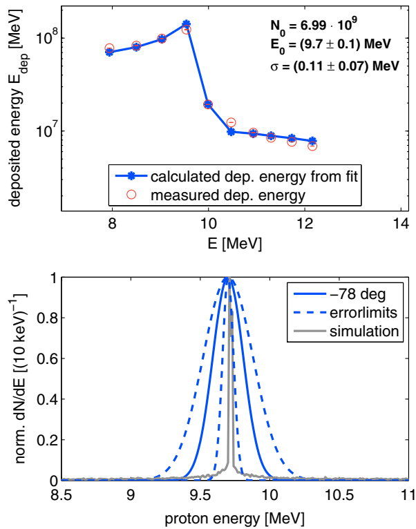
FIG. 5. Shown are the measured deposited energy profile in the RCFs and the calculated one by the fit (upper graph), and the obtained particle spectrum at \Phi_s = -78 \text{ deg} including a simulation reference (lower graph).
