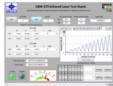
Figure 4: Run time operator interface for the LTS.
