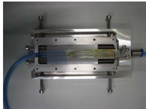
Figure 4: Final tool.
