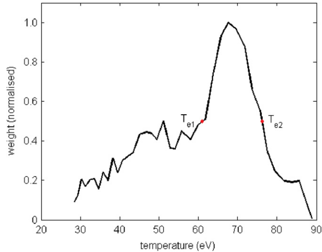
Figure 7. The temperature distribution seeded by the measured spatial intensity distribution incident on the plasma mirror surface. Each temperature is weighted by the incident laser intensity at that point to correlate the position with its influence on the final far field. The temperatures T_{e1} and T_{e2} , as defined in equation (5) are also shown.
