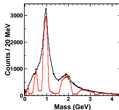
Figure 1: Improved particle identification in the mass spectrum. Initial mass spectrum after the track reconstruction and p-value cut at pv > 0.05 is shown in black line. The red line shows the improved mass spectrum of the track reconstruction when the probability of identification is used by setting a minimum probability.
