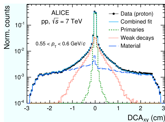
Fig. 10 Proton \text{DCA}_{xy} distribution in the range 0.55 < p_T < 0.60 GeV/c together with the Monte-Carlo templates for primary protons (green dotted line), secondary protons from weak decays (red dotted line) and secondary protons produced in interactions with the detector material (blue dashed line) which are fitted to the data. The light blue line represents the combined fit, while the black dots are the data
