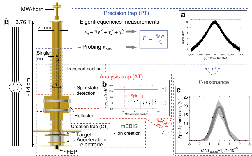
Figure 2 | The g -factor experiment for highly charged ions. The triple Penning-trap set-up (gold) comprises: (i) The PT with a homogeneous magnetic field to determine the frequency ratios \Gamma^* by measuring the three motional eigenfrequencies and probing the Larmor frequency. (ii) The AT to detect the spin-state of the valence electron. (iii) The Creation trap (CT) for ion creation within a miniature electron beam ion source (mEBIS). To enhance the production rate of ^{48}\text{Ca} ions, an enriched calcium target is used with the following isotope composition: ^{40}\text{Ca} : 78.77%, ^{42}\text{Ca} : 3.02%, ^{43}\text{Ca} : 0.62%, ^{44}\text{Ca} : 9.55%, ^{46}\text{Ca} : 0.02% and ^{48}\text{Ca} : 8.02%. The set-up is placed in a cryogenic ( T = 4.2\text{ K} ) ultra-high vacuum chamber ( P < 1 \times 10^{-16} mbar). In a the axial resonator noise spectrum is shown including the dip-signal of a thermalized single ^{48}\text{Ca}^{17+} ion. In b the spin-state of the ^{48}\text{Ca}^{17+} ion is detected as an axial frequency jump at an absolute axial frequency of \nu_{z,\text{off}} = 412.4\text{ kHz} . In c the spin-flip probability is shown in dependence of the measured \Gamma^* -values, scaled by the final central \Gamma value \Gamma_{\text{mean}} = 5138.837\,974\,37 (58). The black points represent binned data to guide the eye. This data binning is not relevant for the Gaussian maximum-likelihood (ML) fit, shown in red. The dark grey-shaded area illustrates the uncertainty of \Gamma_{\text{mean}} and the bright grey area represents the binomial errors considering the amount of cycles of binned data and the probability of the ML fit. Error bars represent the uncertainties of each single axial frequency measurement point is related to the 1 sigma standard deviation.
