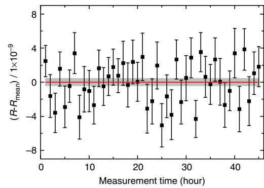
Figure 3 | Data sets of the cyclotron-frequency ratio measurements R_{1h} of ^{48}\text{Ca}^{17+} and ^{12}\text{C}_4^{17+} at SHIPTRAP. The red line and the grey-shaded band illustrate the mean ratio R_{\text{mean}} and the s.d. For details on the plotted error bars see text.
