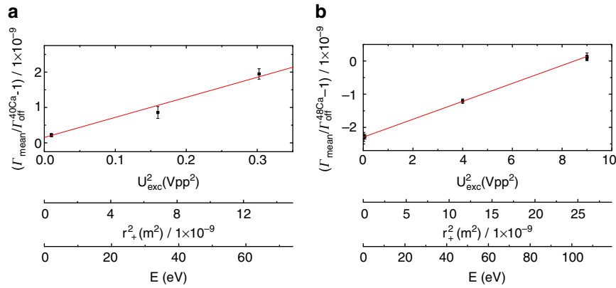
Figure 5 | \Gamma -resonances at different modified cyclotron energies. We measure for both isotopes various \Gamma -resonances at different modified cyclotron energies. Here we show the extracted mean values \Gamma_{\text{mean}} , normalized by the constant values: \Gamma_{\text{off}}^{40\text{Ca}} = 4,282.429538772 in a and \Gamma_{\text{off}}^{48\text{Ca}} = 5,138.837973696 in b in dependence of the modified cyclotron energy, which is proportional to the squared amplitude U_{\text{exc}} of the first excitation pulse. The slope is mainly given by the relativistic mass shift in the cyclotron frequency. The indicated error bars illustrate the statistical uncertainty of the weighted maximum-likelihood fit (see the dark-shaded area in Fig. 2c).
