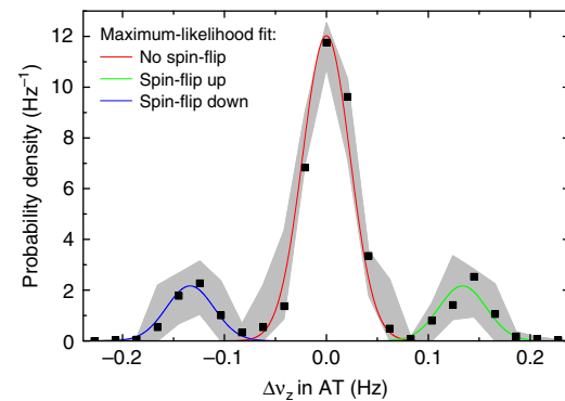
Figure 4 | Probability density of the measured axial frequency differences in the AT. \Delta\nu_z is the axial frequency difference of subsequent measurements in the AT with 30 s spin-flip drives in between. From a maximum-likelihood (ML) fit, which combines three Gaussian distributions (red: no spin-flip (sf), green: spin-flip up, blue: spin-flip down), the following parameters are extracted: the spin-flip rate: 26.5%, the frequency jitter: \sigma_{\Delta\nu_z} = 25 mHz and the axial frequency jump due to a spin-flip: \Delta\nu_z^{\text{sf}} = 140 mHz.
