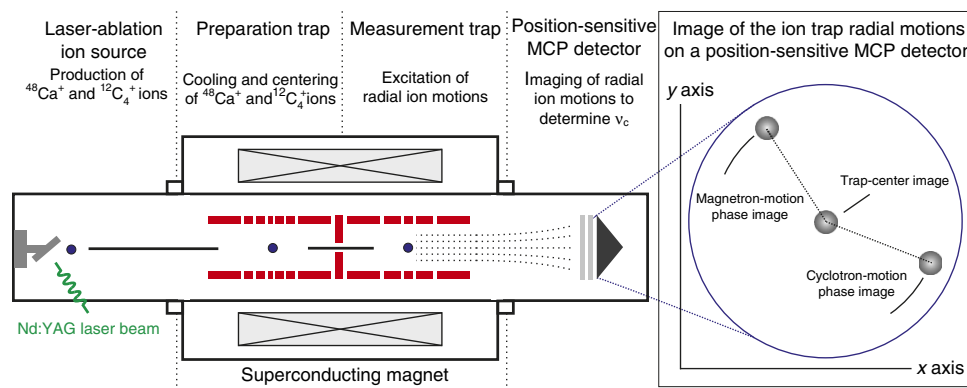
Figure 1 | Offline configuration of the Penning-trap mass spectrometer SHIPTRAP. The set-up contains a laser-ablation ion source, two Penning traps, one for the preparation of the ion (cooling and centering), the other for the frequency measurement process and a position-sensitive multi-channel plate (MCP) detector for a radial resolution of the ion position. The novel PI-ICR is alternately applied to small clouds of ^{48}\text{Ca}^+ and ^{12}\text{C}_4^+ ions, determining their respective cyclotron frequencies.
