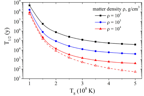
Fig. 7. Estimated half-lives for the allowed electron capture by the ^{123}\text{Te} excited state at 159 keV with the formalism of [15] in dependence on temperature in units of 10^8 K and on density in \text{g/cm}^3 . The dashed curve shows the total half-lives which include the capture of free electrons for \rho = 10^4 \text{g/cm}^3 .
