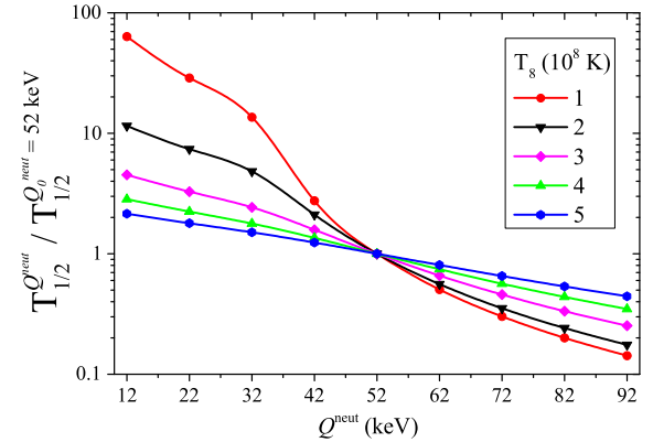
Fig. 3. Effective half-life of ^{123}\text{Te} in dependence on Q^{\text{neut}}_0 -value. All the data points are normalized to the effective half-life of ^{123}\text{Te} with Q^{\text{neut}}_0 = 52 \text{ keV} . The half-lives are calculated with matter density \rho = 10^3 \text{ g/cm}^3 and for various stellar temperatures in units of 10^8 \text{ K} .
