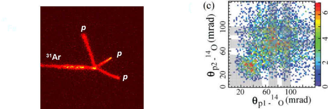
Fig. 12: Exotic radioactive decays: Left: 3-proton-emission following beta-decay in ^{31}\text{Ar} observed with the Optical-TPC in an FRS experiment (published in [Lis-15]). Right: The measured correlation plot of 2p decays of ^{16}\text{Ne} states populated in a neutron knockout from ^{17}\text{Ne} projectiles. Shaded areas of the circular sector and bands indicate the true 2p decay of the ground state and the sequential decays of excited states via the intermediate ^{15}\text{F} states.
