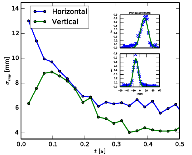
Figure 4. Beam size development (Inserted: Vertical and horizontal beam profiles at t=0.24s )
