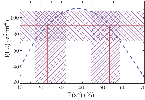
Fig. 7. Transition probabilities B(E2, 1/2^- \rightarrow 5/2^-) as a function of the s -shell occupation, P(s^2) , in ^{17}\text{Ne} (g.s.). The solid line gives experimental B(E2) value and the hatched zone shows the 1\sigma deviation from this value. The dashed line represents calculations from Ref. [21].
