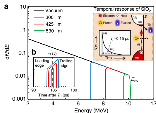
Figure 1 | Ultrafast proton pulse metrology in SiO 2 . The dashed inset shows a schematic of the intraband dynamics and temporal response of an excited electron in a -SiO 2 . VB and CB are the valance and conduction bands, respectively, and E is the energy. Exciton formation provides the ultrafast de-excitation pathway for electrons in the CB 8 . The time constant for exciton formation is \sim 0.15 ps (refs 8,20). (a) Schematic of a TNSA proton spectrum (black trace) represented by a truncated exponential, with a proton temperature T = 2 MeV and a high-energy spectral cutoff E_{co} = 10 MeV. The coloured traces show the bandwidth of the original spectrum that remains after proton stopping at different depths D , in bulk SiO 2 (density 2.66 \text{ g cm}^{-3} ) from stopping and range of ions in matter (SRIM) calculations 24 (see Methods for more details). This returns a continuously decreasing bandwidth with respect to D (up to the stopping depth for E_{co} , here \sim 570 \mu\text{m} ). The proton pulse duration \tau(D) (b) is then simply the difference in time of flight for vacuum propagation (chosen here to be 5 mm) plus D for both the leading and trailing (high and low kinetic energy) edges of the remaining proton bandwidth. This illustrative schematic shows only the cumulative bandwidth narrowing of the originally broadband spectrum to reveal how short pulses can in principle be retrieved. It does not account for other aspects of the TNSA mechanism, such as energy-dependent cone narrowing 12–14 critical for determination of the detailed proton pulse profile for a particular D .
