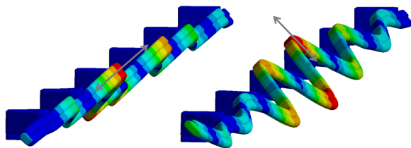
Figure 1: Mechanical eigenmodes of the electrodes
