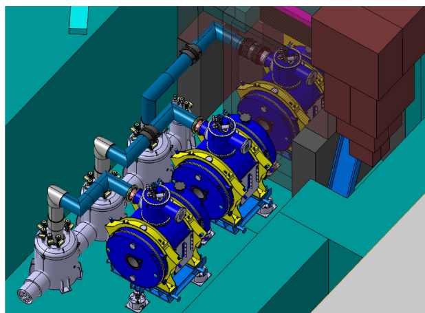
Figure 1: Each cryo-module is operated by an individual feedbox as shown for some short multiplets located in the Pre-Separator.
