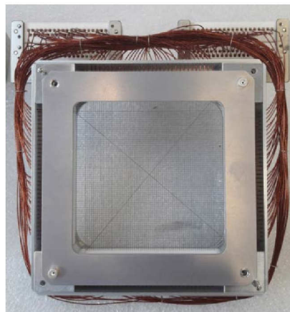
Figure 3: Prototype of SEM-Grid detector
