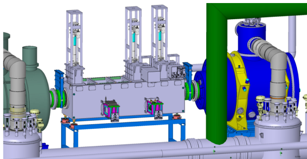
Figure 2: Focal plane chamber at PPF2 with some of its beam instrumentation inserts.
