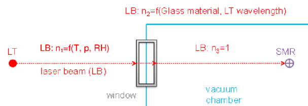
Figure 2: Splitting the distance in separate parts regarding the refractive index of the different optical media
