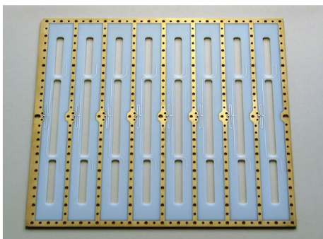
Figure 1: Prototype slotline electrode plate (signal side).
