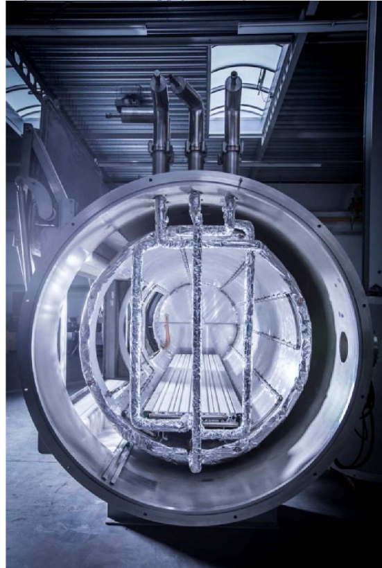
Figure 5: Helium Supply Facility ( HeSu)
