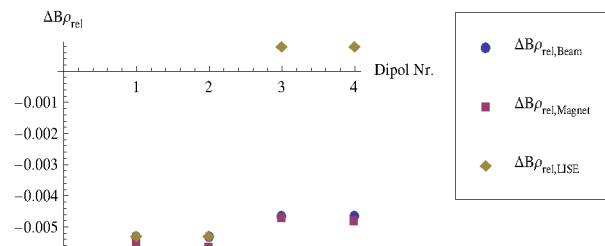
Figure 1: \Delta B\rho_{rel} for ^{238}\text{U}^{92+} setting
