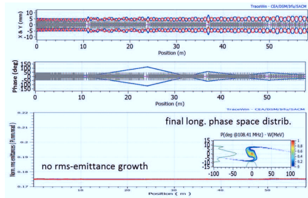
Figure 4: Simulated transverse (upper) and longitudinal (middle) rms-envelopes and transverse rms-emittances (lower) along the beam line of the new post-stripper Alvarez-type DTL for provision of ^{238}\text{U}^{28+} at 3.3 MeV/u at low current.
