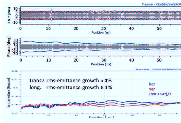
Figure 3: Simulated transverse (upper) and longitudinal (middle) rms-envelopes and transverse rms-emittances (lower) along the beam line of the new post-stripper Alvarez-type DTL for provision of 15 mA of ^{238}\text{U}^{28+} at 11.4 MeV/u.
