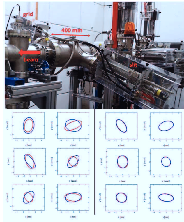
Figure 2: ROTating System for Emittance measurements ROSE (upper). Measured rms-ellipses of the transverse projections as measured at ROSE behind the triplet (lower left) and from back-transformation to the entrance of the skew triplet (lower right). Measurements were done for two different skew triplet settings.
