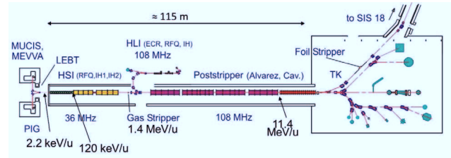
Figure 1: The UNILAC (UNiversal Linear ACcelerator) at GSI.
