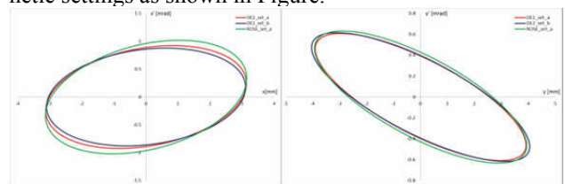
Figure 7: Comparing the horizontal and vertical emittance of a 1.4 \text{ MeV/u Ar}^{9+} beam in front of the doublet measured with ROSE and existing scanners for different quadrupole settings.
