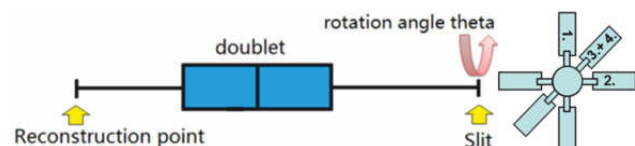
Figure 2: To obtain the beam matrix C at the reconstruction point all four emittance values are measured using ROSE behind a magnetic doublet.
