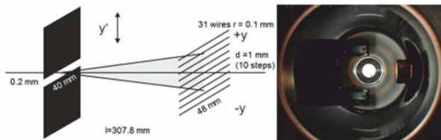
Figure 4: Schematic figure and photo of the slit and grid.
