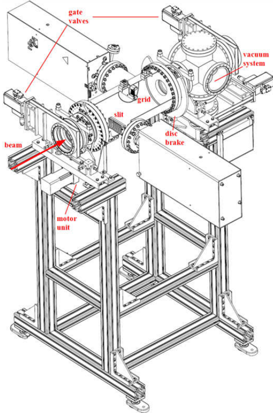
Figure 3: The ROSE detector system
