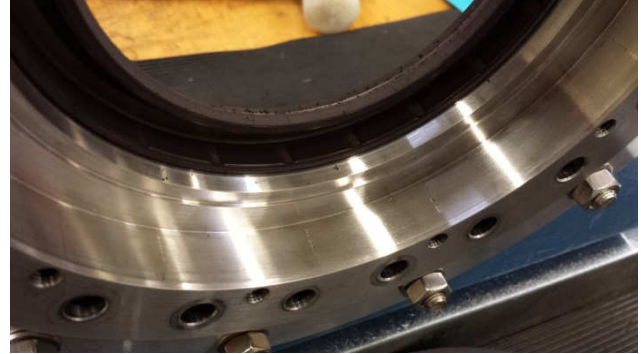
Figure 6: Damaged seal after some tens of dry turns.
