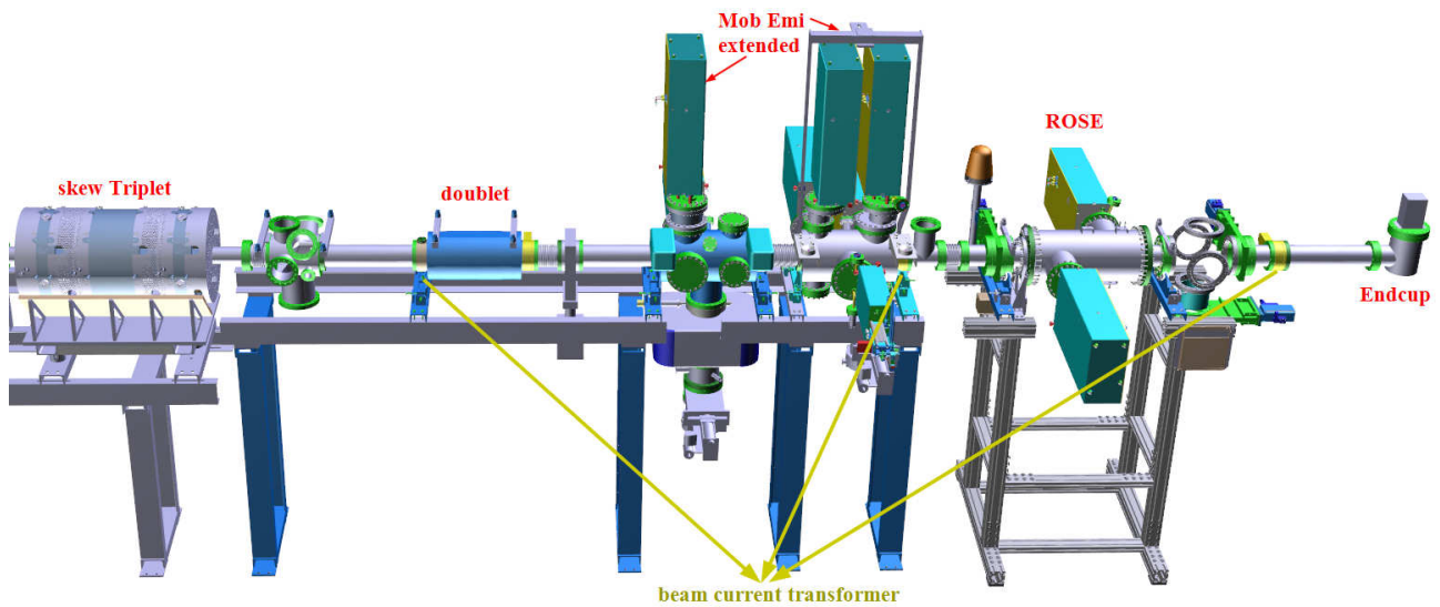
Figure 8: Experimental setup used for the ROSE commissioning.
