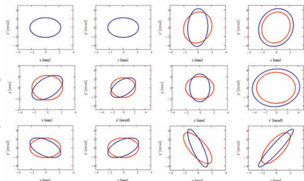
Figure 1: Simulation of an initially uncoupled (red) and coupled (blue) ion beam (left) through a solenoid channel (right).
