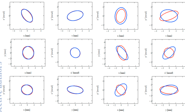
Figure 9: Experimental proof for ROSE capability to measure the 4d beam matrix.
