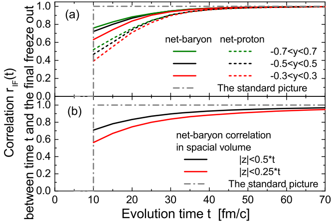
Fig. 1. [Color online.] (a) Correlation of the finally observed net-proton and net-baryon number in different rapidity intervals with an earlier time t in that same rapidity interval. Results for central collisions of Au+Au at a beam energy of \sqrt{s_{NN}} = 200 GeV are shown. (b) Same as in (a), just in this case we show the correlation for a defined spatial volume, constrained by z < v_z \cdot t rather than rapidity.
