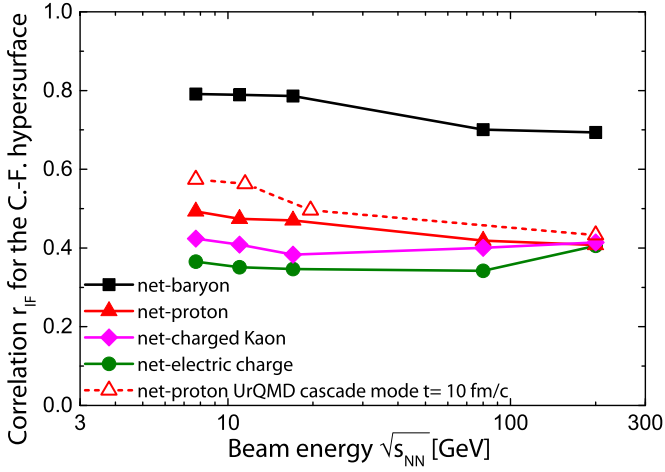
Fig. 3. [Color online.] Correlation of the finally observed net-charge, net-kaon, net-proton and net-baryon number in the rapidity interval -0.5 < y < 0.5 , at the Cooper-Frye hypersurface, with the final net-charge density as a function of beam energy.
