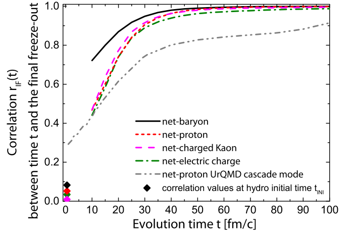
Fig. 2. [Color online.] Correlation of the net-charge, net-kaon, net-proton and net-baryon number in the rapidity interval -0.5 < y < 0.5 with an earlier time t in that same rapidity interval.
