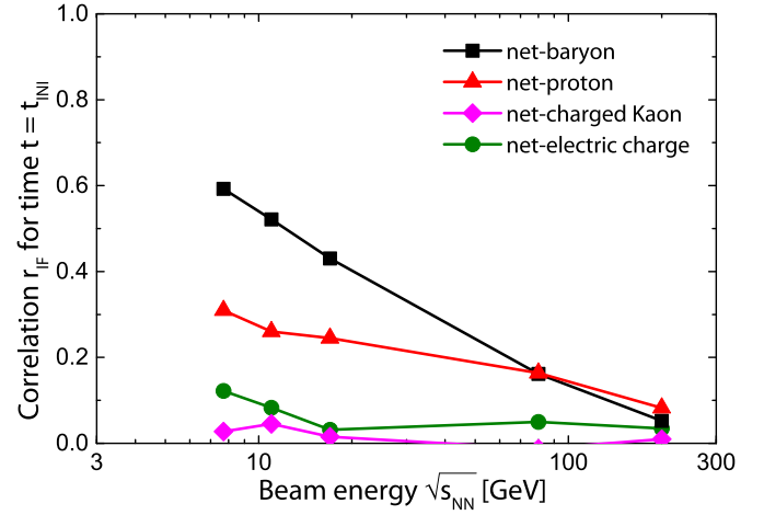
Fig. 4. [Color online.] Correlation of the net-charge, net-kaon, net-proton and net-baryon number in the rapidity intervals -0.5 < y < 0.5 at the initial hydro time with the final net-charge density in that same rapidity interval, as a function of beam energy. Note that the additional decorrelation, with respect to Fig. 3 stems from the enforced local equilibration in the fluid dynamical evolution and the Cooper-Frye sampling at its end.
