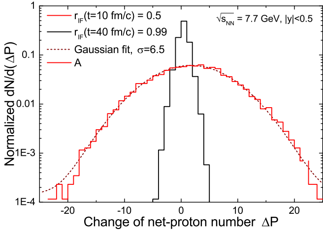
Fig. 5. [Color online.] Probability distribution of the change of the net-proton number in the time interval between t = 10 fm/c (red line), t = 40 fm/c (black line) and the last scattering. We show results for \sqrt{s_{NN}} = 7.7 GeV. The corresponding correlation values r_{IF}(t) are 0.5 for t = 10 and 0.99 for t = 40 fm/c. We also fitted the distribution for t = 10 fm/c with a Gaussian function and obtained a width \sigma = 6.5 which is close to the width of the final net-proton distribution \sigma_{final} = 7.5 .
