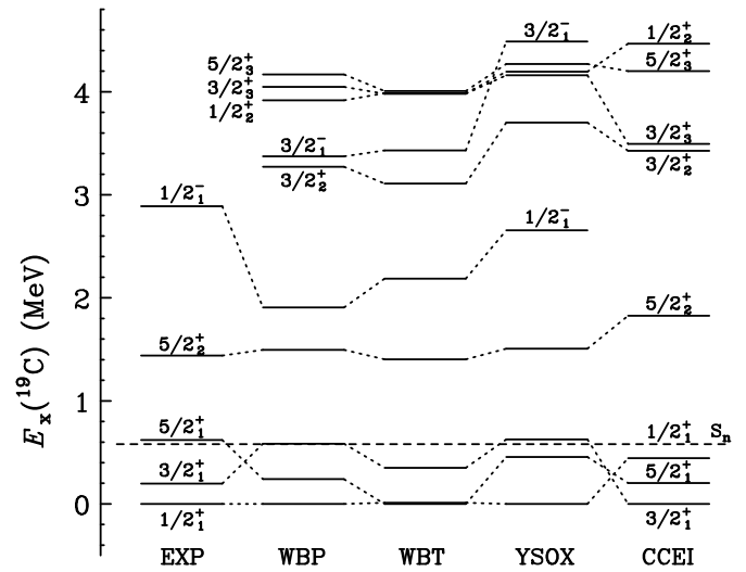
Fig. 4. Energies of states observed in ^{19}\text{C} (EXP: present work and Refs. [19–21,24]) as compared to shell-model predictions ( E_x < 5 MeV) for states with J^\pi \leq 5/2^+ and 3/2^- using the WBP, WBT [38], YSOX [12], and CCEI [10] interactions. The latter are confined to 1s0d -shell states only.
