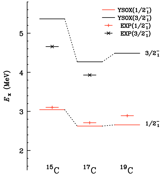
Fig. 3. (Color online.) Excitation energies of the 1/2_1^- (red) and 3/2_1^- (black) levels in ^{15,17}\text{C} [49–51] compared with shell-model calculations employing the YSOX interaction (see text). In the case of ^{19}\text{C} the \ell = 1 resonance observed here at 2.89 MeV is displayed together with the shell-model predictions.
