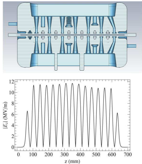
Figure 2: CST model for the 15-gap CH cavity (top) and the calculated accelerating electrical field along the cavity (bottom).
