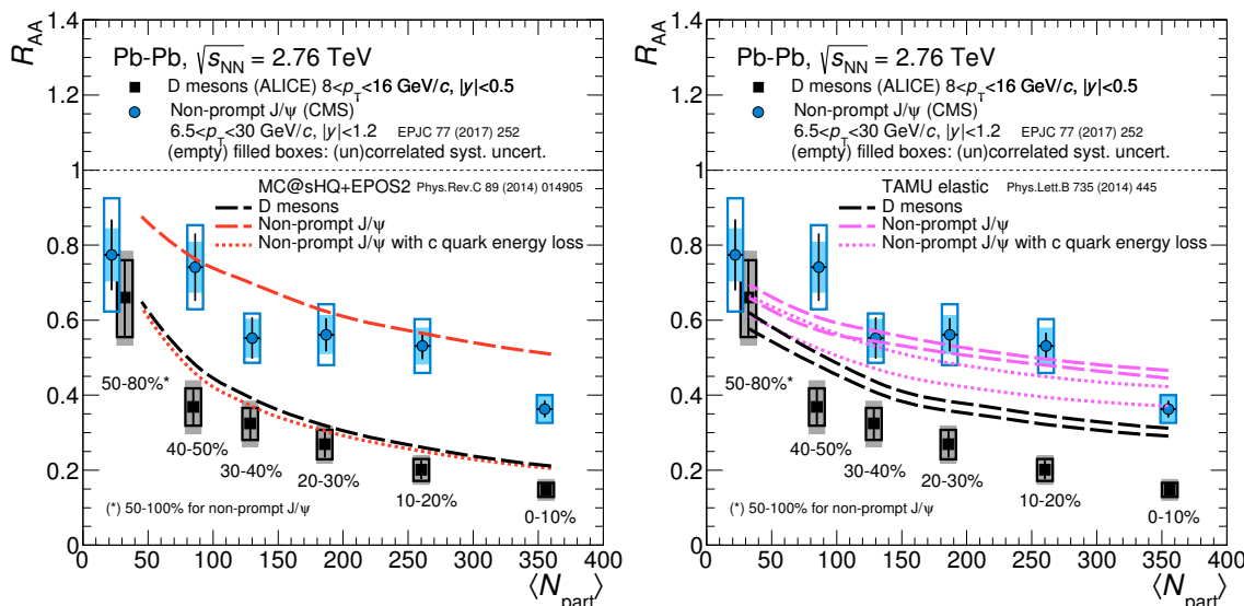
Figure 3. Comparison of the R_{AA} measurements with the MC@SQ+EPOS2 model [5] including radiative and collisional interactions (left) and with the TAMU elastic model [6] including collisional interactions via in-medium resonance formation. For both models, results for the case in which the b quark interactions are calculated using the c quark mass are shown as well [7]. In the right-hand panel, the band between lines with the same style represents the theoretical uncertainty. This figure updates figure 5 of [1].
