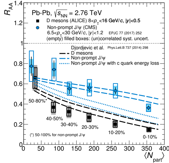
Figure 2. Comparison of the R_{AA} measurements with the calculations by Djordjevic et al. [4] including radiative and collisional energy loss. Lines of the same style enclose a band representing the theoretical uncertainty. For non-prompt J/\psi mesons in 6.5 < p_T < 30 GeV/c [2] the model results for the case in which the b quark interactions are calculated using the c quark mass are shown as well [7]. This figure updates figure 4 (right) of [1].
