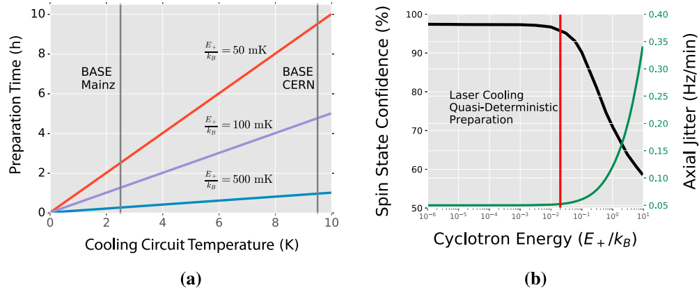
Figure 1. (a) Approximate preparation times required to prepare an (anti-)proton at a cyclotron energies of E_+ = 50 \text{ mK}/k_B (orange), 100 \text{ mK}/k_B (purple), and 500 \text{ mK}/k_B (blue). The vertical grey lines represent the different conditions for the BASE CERN antiproton experiment and the BASE Mainz proton experiment (22). (b) Illustration of the spin state detection fidelity and the axial frequency fluctuation as a function of the cyclotron energy E_+ = 0.5 \text{ K}/k_B . At radial energies below 0.1 \text{ K}/k_B we achieve a spin state identification fidelity close to 100 %. Currently, we use particles with energy E_+ = 0.6 \text{ K}/k_B , prepared by resistively coupling to a detector at \approx 2 \text{ K} (Mainz) and \approx 9.5 \text{ K} (CERN).
