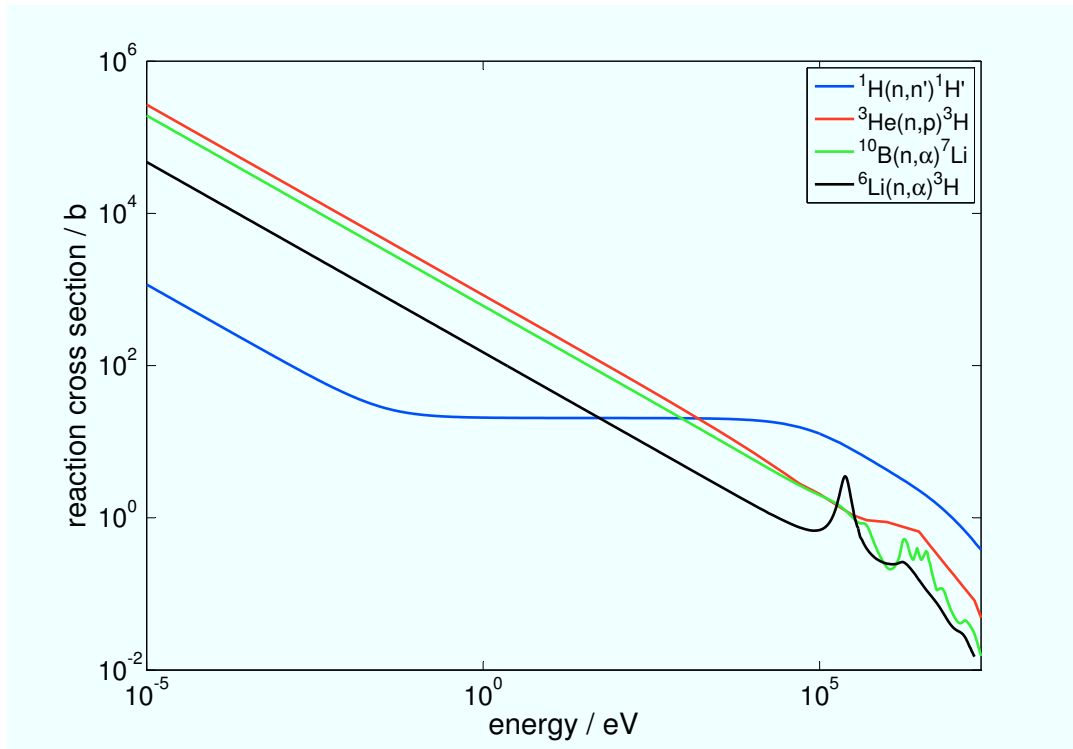
Figure 4.1.: Comparison of the neutron reaction cross sections given above. The data was obtained from references [102] and [150].
