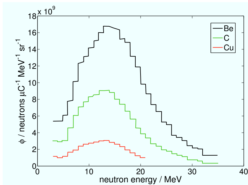
Figure 3.3.: Comparison of the neutron flux originating from different catcher materials. The data is taken from the experimental results of reference [107].
