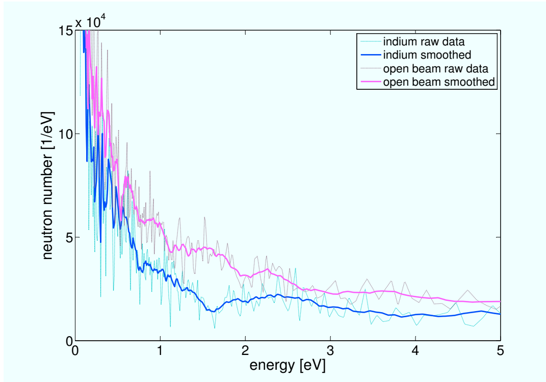
Figure 6.10.: Comparison of open beam measurements averaged over five shots (violet) and measurements with a 5 mm indium sample averaged over three shots (blue). The dotted and solid lines are the raw data and a smoothing by a moving average over 10 data points, respectively.
