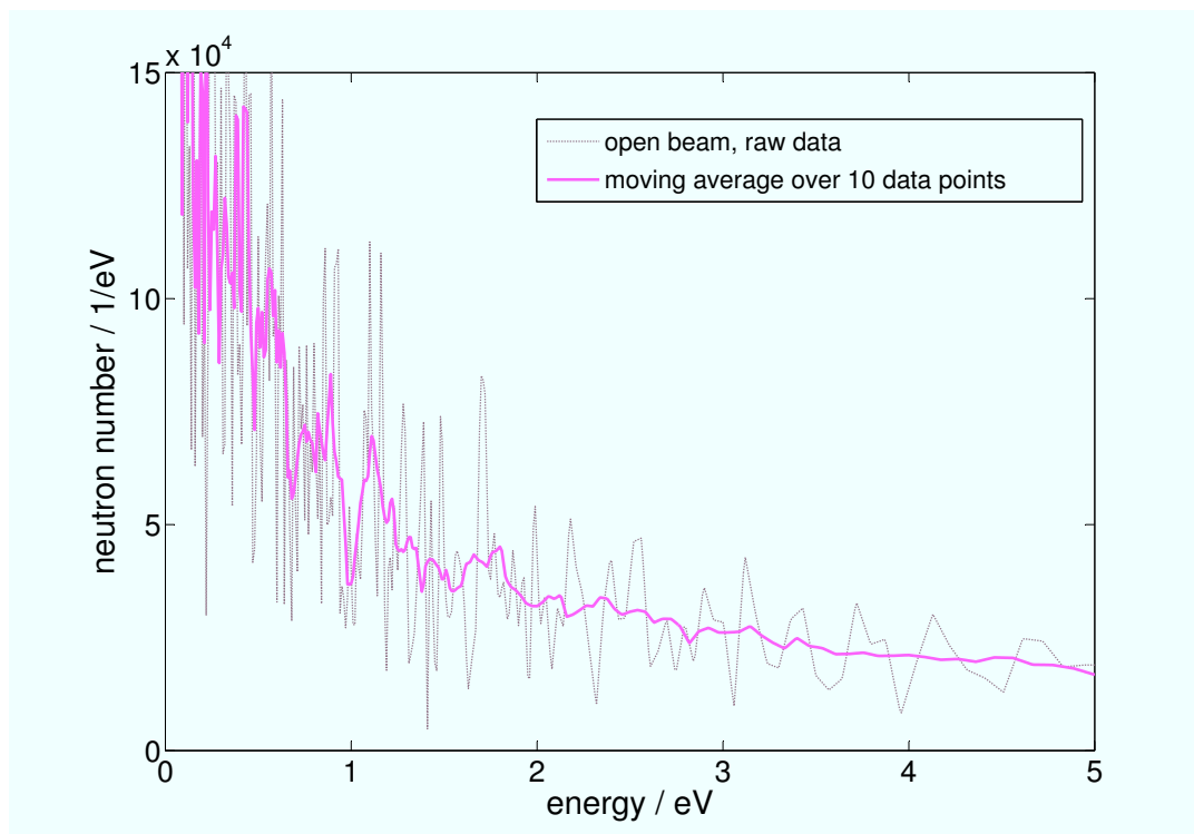
Figure 6.7.: Energy spectrum of an open beam measurement (dotted line). The signal was smoothed by applying a moving average over 10 data points (solid line).
