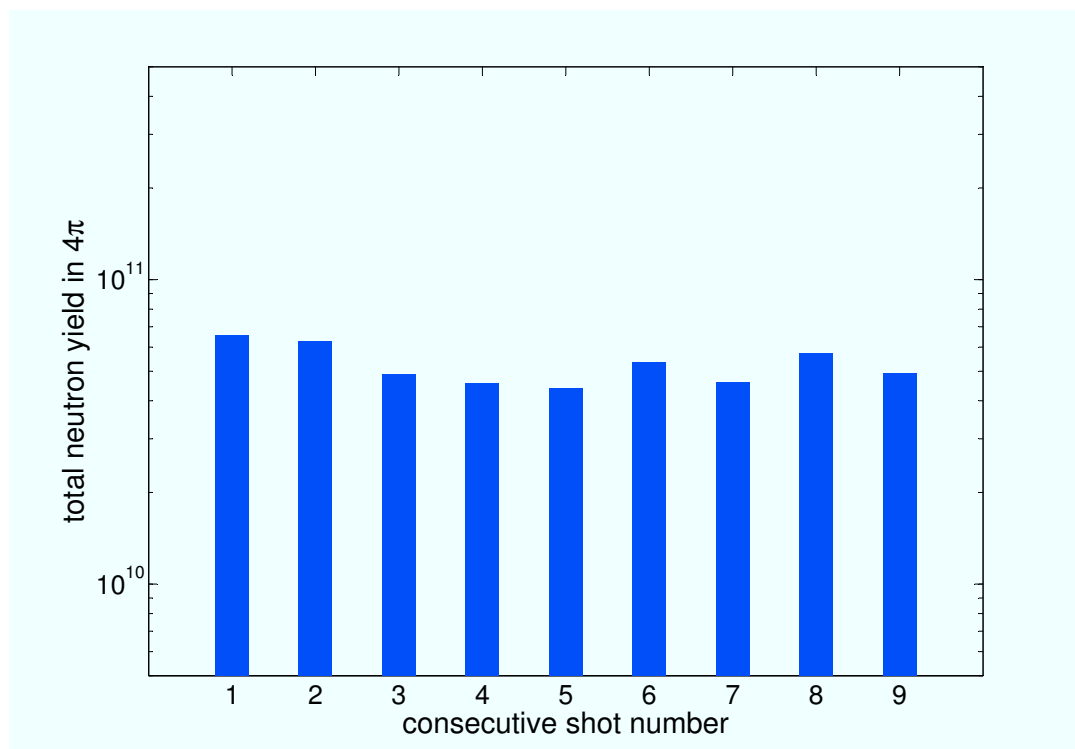
Figure 5.7.: Total neutron yield for every shot of the experiment with a catcher behind the primary target.
