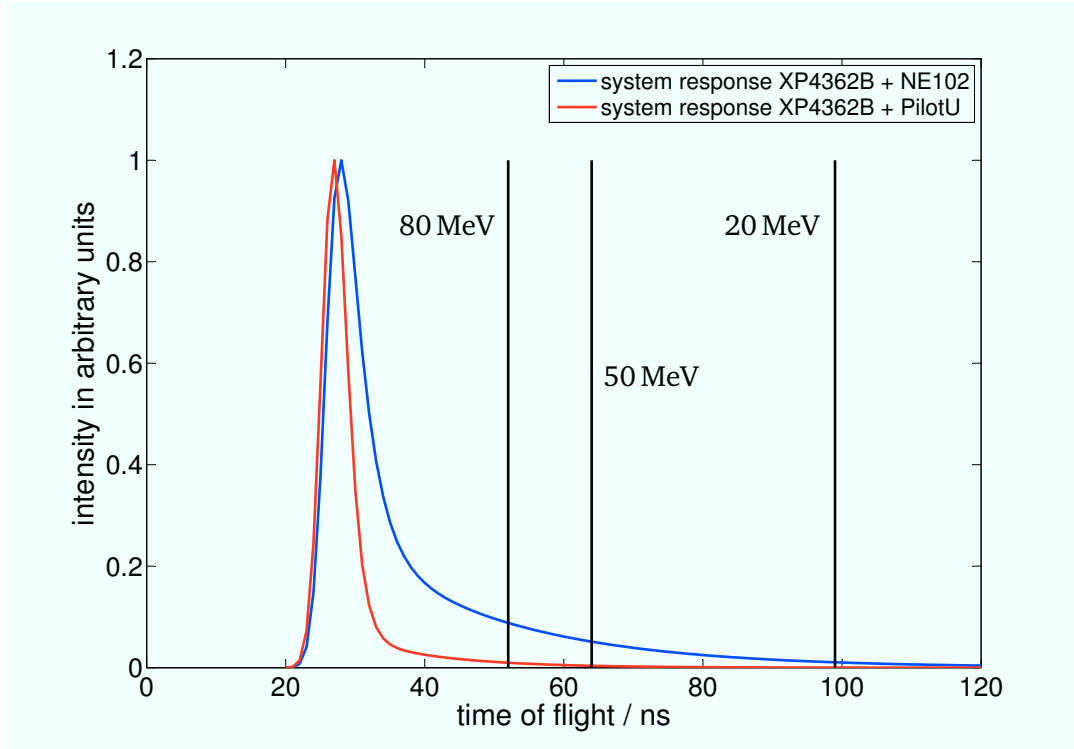
Figure 8.5.: Temporal system response calculated by convolution of the time response of the scintillators NE102 (blue) and PilotU (red) with a Photonis XP4362B PMT. The temporal characteristics of the components were obtained from references [159, 161, 185–187]. The black lines mark arrival times for neutrons with different energies. The calculation is based on the experimental setup of the Trident experiment introduced in section 6.1 for a detector at a distance of 6 m from the neutron source. t = 0 s is defined as the time of the laser shot.
