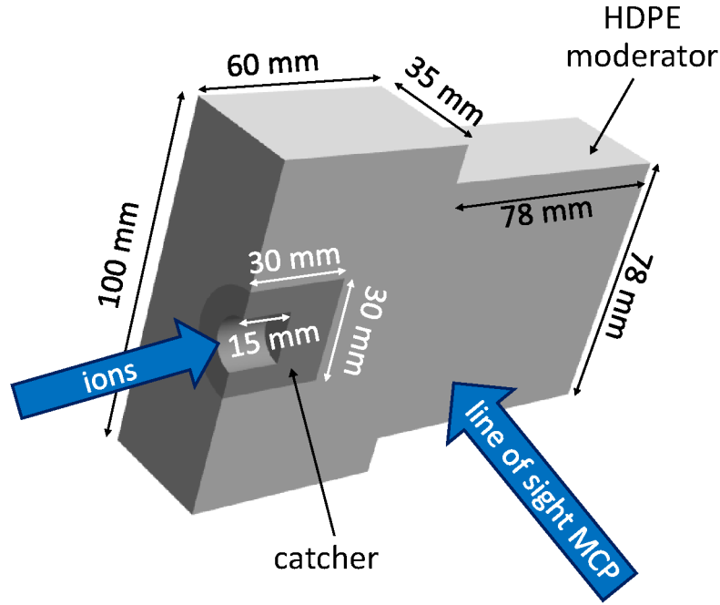
Figure 6.4.: Sketch of the HDPE moderator and the beryllium catcher, which had a hole drilled into it to reflect backscattered neutrons.
