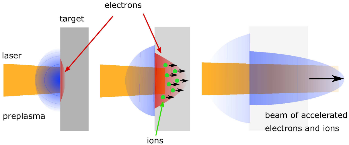
Figure 2.4.: Sketch of ion acceleration in the relativistic transparency regime. (left) The main pulse of the laser accelerates the electrons at the critical density to relativistic energies. (center) Due to the relativistic mass increase as well as the expansion of the target, the target gets relativistically transparent to the laser. Inside the target volume, the electrons transfer their energy to the ions which are accelerated, while themselves regain their energy by interaction with the laser field. (right) The target expands to the point where it gets classically underdense and the acceleration stops.
