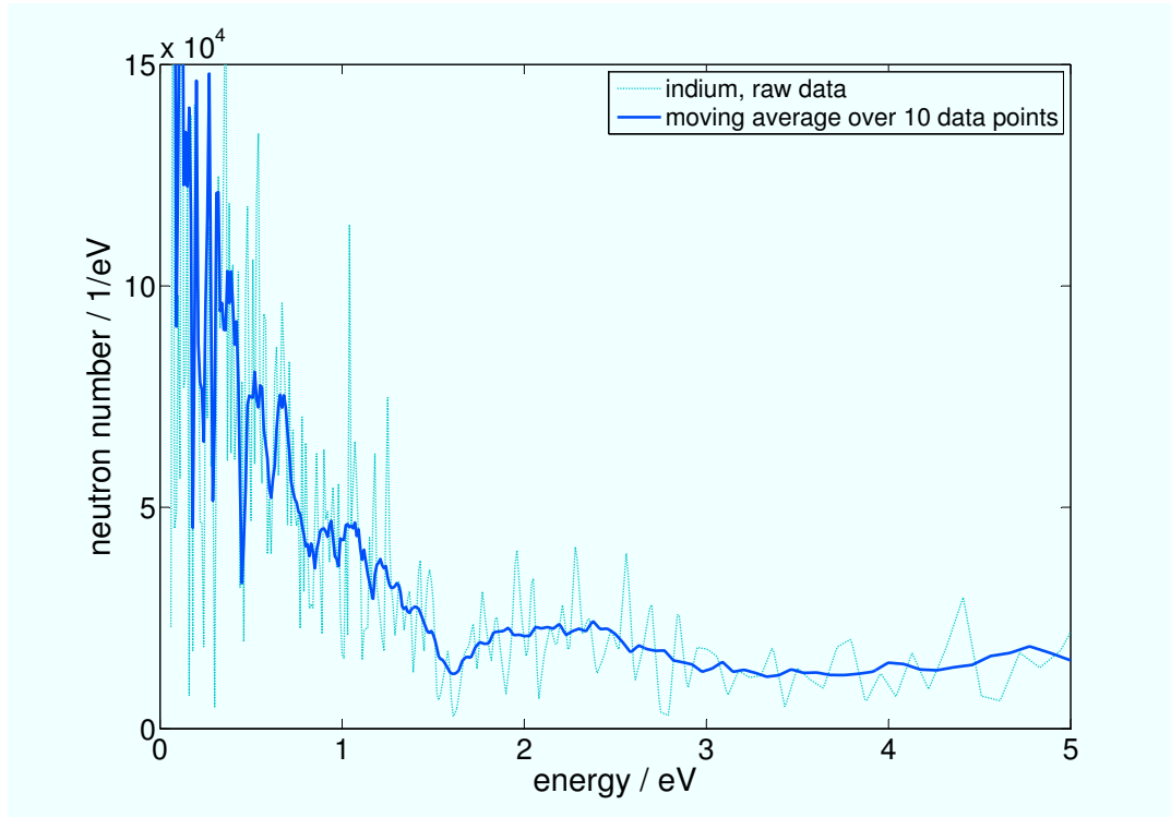
Figure 6.8.: Single shot measurement of the neutron spectrum (dotted line) conducted with the boron-doped MCP detector placed at 90^\circ with a 5 mm ^{115}\text{In} sample directly in front of the detector. The solid line represents a smoothing of the dotted curve by a moving average over 10 data points.
