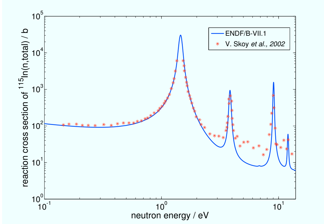
Figure 3.7.: Total reaction cross section of neutrons with ^{115}\text{In} within an energy interval from 0.1 to 15 eV. The solid line shows an ENDF/B-VII.1 calculation taken from reference [102]. The red dots are taken from reference [138].
