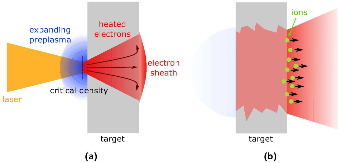
Figure 2.3.: Scheme of the TNSA mechanism. (a) The main pulse of the laser accelerates electrons in the region of the critical density. They propagate through the target and build up a sheath at the rear surface, which causes an electrostatic field. (b) This field ionizes the atoms at the target rear side, which subsequently get accelerated.
