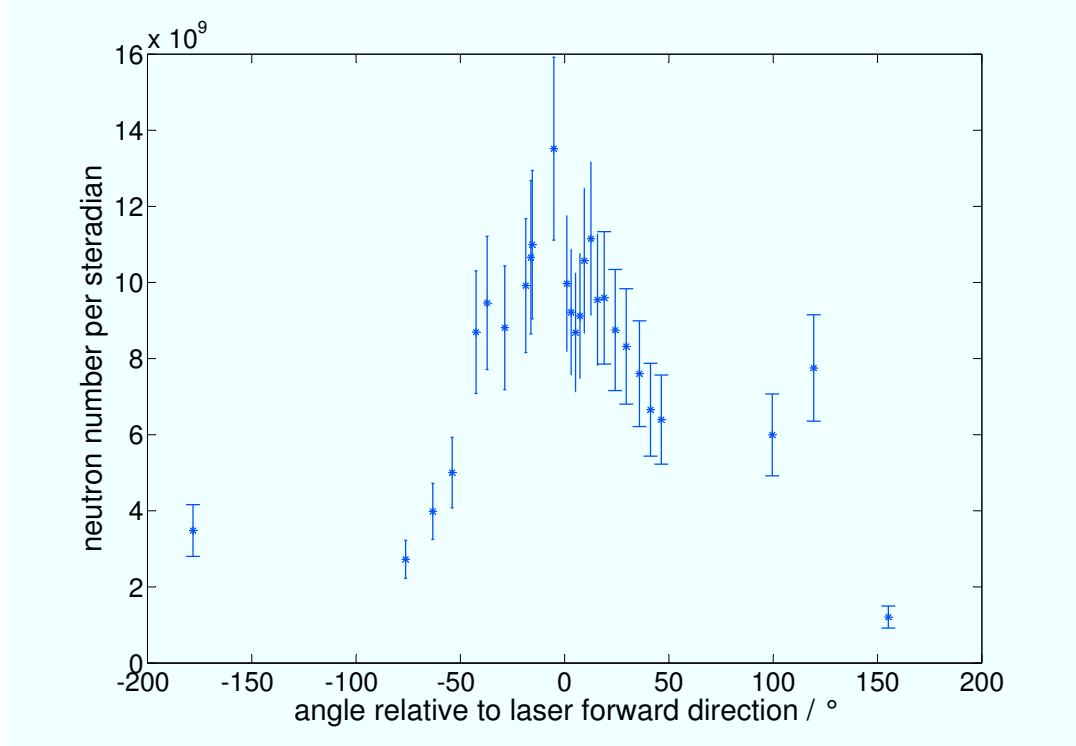
Figure 5.6.: Detailed angular neutron distribution from a CD target and a beryllium catcher measured with 27 bubble detectors simultaneously at the PHELIX laser system. For clarity reasons, the angle uncertainty of 2^\circ is not shown in the graph.
