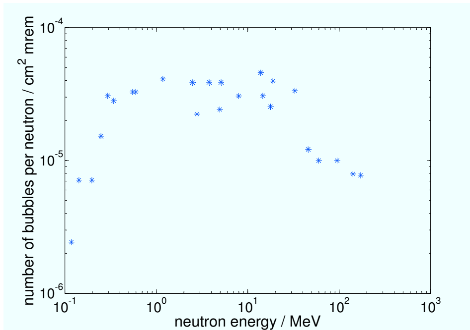
Figure 4.3.: Sensitivity of a bubble detector with a response of one bubble per mrem. The data was taken from references [151, 152].
