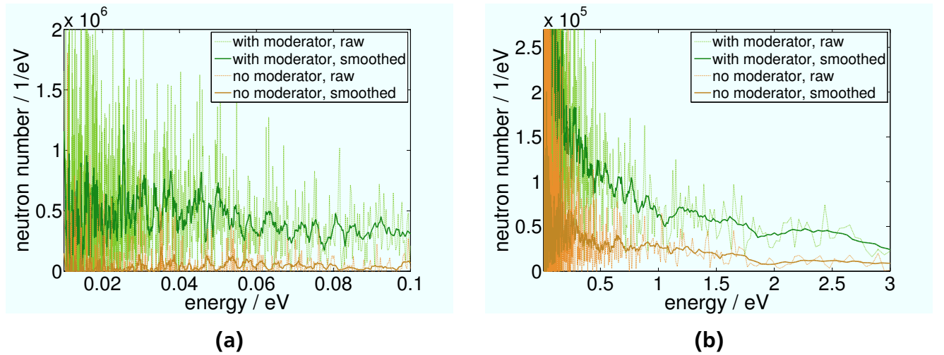
Figure 6.5.: Comparison of exemplary measurements with (green) and without (brown) a moderator displayed for (a) thermal energies and (b) an energy range around the indium resonance at 1.46 eV. The data was obtained with the boron-doped MCP detector from Nova Scientific [146, 163]. Dotted lines show the raw signal, which was smoothed with a moving average over 10 data points (solid lines).
