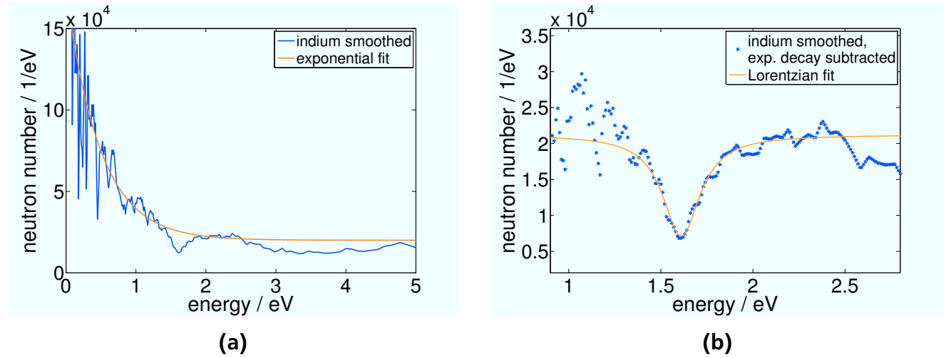
Figure 6.9.: (a) Exponential fit to the neutron spectrum f_{\text{exp}}(E) = A \cdot e^{-BE} + C with parameters A = (1.541 \pm 0.157) \cdot 10^5 \text{ eV}^{-1} , B = (2.070 \pm 0.234) \text{ eV}^{-1} , and C = (2.003 \pm 0.205) \cdot 10^4 \text{ eV}^{-1} . (b) Enlargement of the negative peak shown in Figure 6.8 with subtracted fit of the exponential decay and shift by C as it is described in the text. The dots show the smoothed data of the result. The resonance was fitted with the Lorentzian function given in equation (6.2) (solid line).
