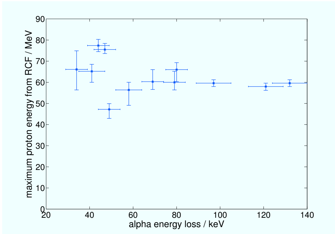
Figure 5.5.: Maximum proton energy from the RCF stack over alpha energy loss. The vertical error bars are given by the energy resolution of the particular RCF stack for each shot. The uncertainty of the energy loss is determined by the measurement during the target characterization.
