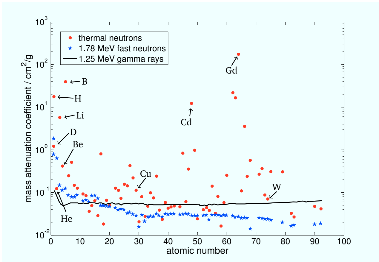
Figure 3.2.: Mass attenuation coefficient of fast (blue) and thermal (red) neutrons with 1.78 MeV and 25 meV, respectively. As a comparison, the attenuation coefficient of gamma rays with an energy of 1.25 MeV (solid line) is displayed. While the attenuation coefficient for gamma rays stays almost constant for different materials, the coefficient for thermal neutrons varies considerably. Fast neutrons show a similar behavior to gamma rays. The plot is adapted from [100] and is based on the NEA data base [101].
