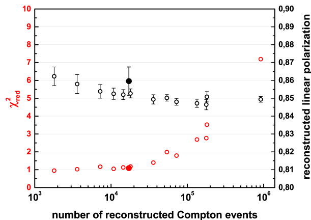
Figure 3. Values of the reduced chi-squared \chi^2_{\text{red}} (red circles) and reconstructed linear polarization (black circles) for multiple simulated data sets with different statistical uncertainties. In addition, points in the plot are displayed for comparison with experimental data points (filled dots), taken from the commissioning experiment at ESR [13].
