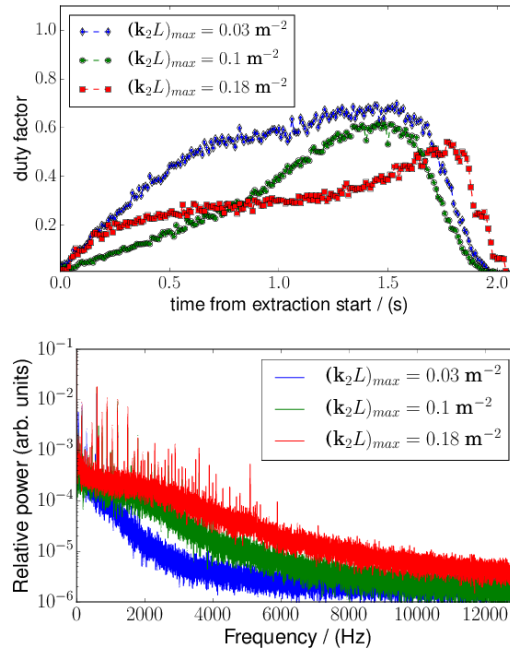
Figure 1. Duty factors as function of time (graph above) and spectral power density of the ripple (graph below) of the spills of coasting beams measured with the maximum strengths of the resonant sextupoles (k_2L)_{\max} = (0.03, 0.1, 0.18) \text{ m}^{-2} .
