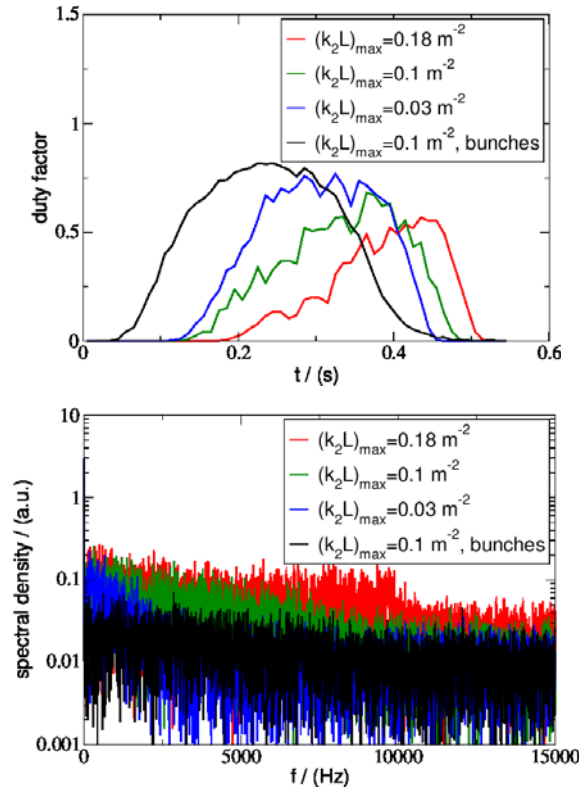
Figure 2. Graph above: Duty factors of the spills simulated for coasting beam for the same sextupole strengths as in Figure 1. Graph: below: Corresponding spill spectra. The black graphs are simulated for the same conditions as the green but the beam was bunched with an rf voltage of amplitude V_a = 2 kV and harmonic number h = 4 .
