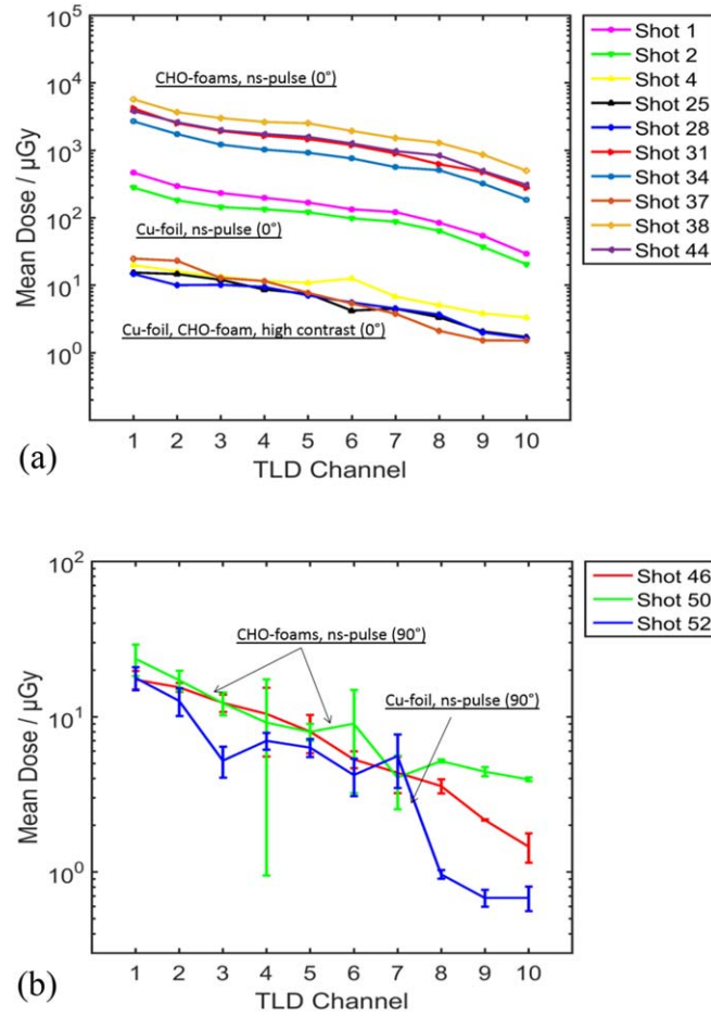
Figure 6. (a) Doses registered by the ten-channel TLD-spectrometer placed in the direction of the laser pulse propagation for shots made at different conditions; (b) same measurements made in the direction perpendicular to the laser pulse propagation.
