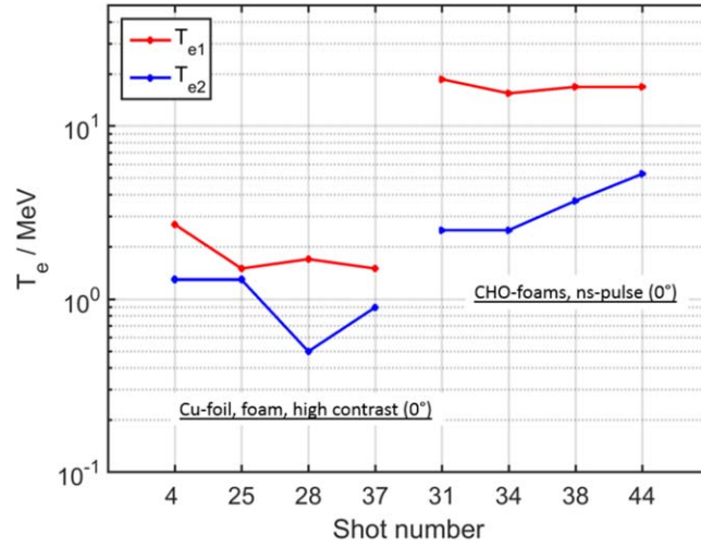
Figure 7. Electron temperatures evaluated from the measured TLD-doses via the best-fit procedure using FLUKA-simulations that accounted for a real geometry of the experimental set-up and the environment and used a two electron temperatures approximation. The best fit was achieved by keeping the deviations of the simulated doses from measured values below 10% for all 10 detector channels simultaneously.
