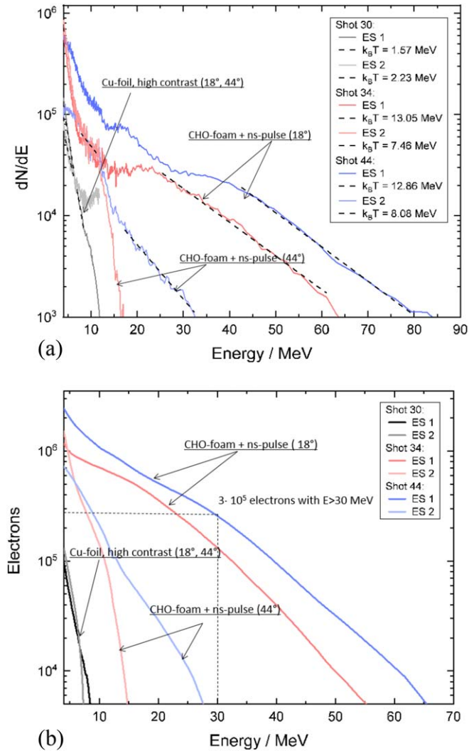
Figure 5. (a) Energy distribution of electrons with energies from 4 up to 80 MeV that entered the spectrometer; (b) evaluated total number of electrons that enter the spectrometer with energies above the given one.
