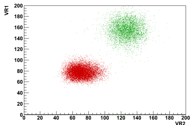
Figure 6: Scatter plot of VR1 versus VR2 for ^4\text{He} (red) and ^{12}\text{C} (green). The VR1 and VR2 variables are measured in terms of number of pixels.
