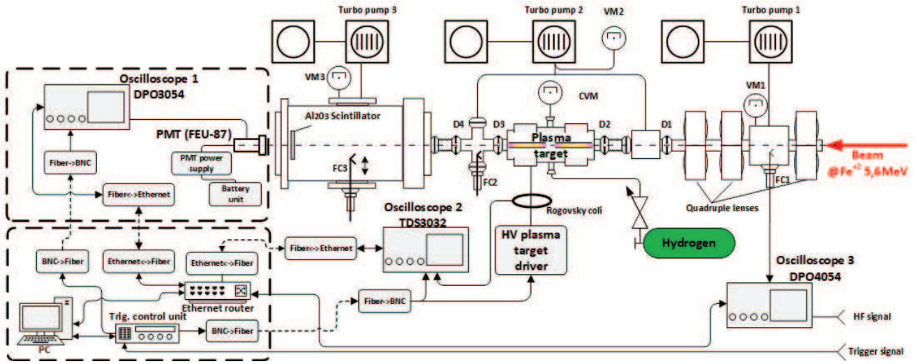
Figure 4: Principal scheme of experimental setup. FC-faraday cup. VM- vacuum meters device. D1-4 differential pumping system diaphragms, CVM –gas independent vacuum meter
