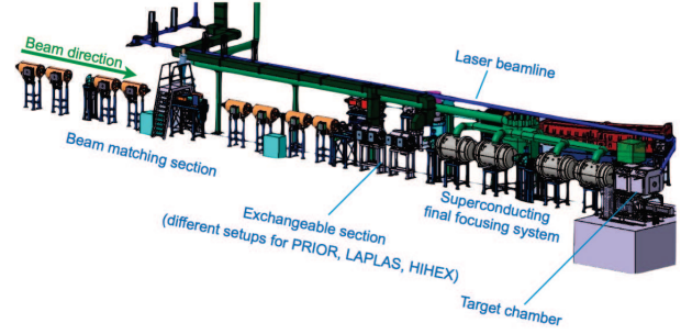
Figure 2: The HED@FAIR beamline in the APPA cave.
