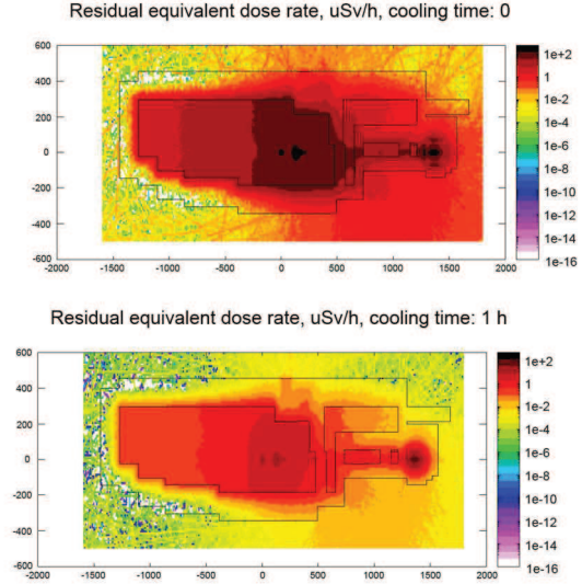
Figure 1: 3D residual equivalent dose maps immediately after the irradiation and for cooling time of 1 hour
