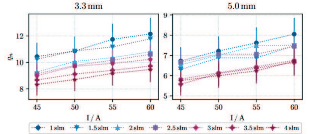
Figure 2: Pressure quotient q_n for different volume flows and currents. Lhs is \varnothing = 3.3 mm, rhs \varnothing = 5 mm
