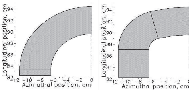
Figure 1: Involutes of the end parts: type 1 is on the left, type 2 is on the right.
