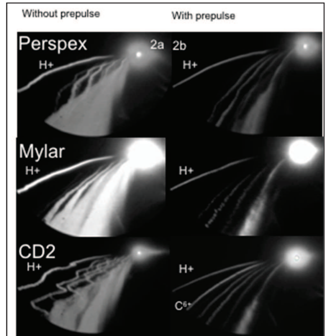
FIG. 1 : Proton beam traces from the Perspex (top), Mylar (center), CD2 (bottom) target front surface, showing the wiggling of the beam for the target kept at best focus, a) without pre-pulse (left), and b) with pre-pulse (right). A comparison of the wiggling of traces shows that with pre-pulse, there is a significant
