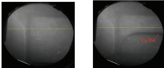
Figure 2: Proton radiography images of Xe target in static (left) and in dynamic process (right, detonation wave propagates from bottom to top). Transmission profiles taken along yellow lines.
