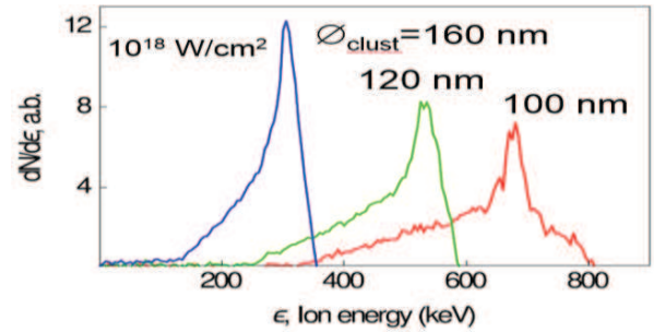
Figure 2. Spectra of impurity cluster ions obtained by 3D PIC simulations (laser: 2 \omega , 16 mJ, \sim 10^{18} W/cm 2 ) [2]
