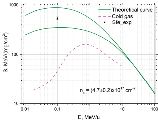
Figure 6. Comparison of experimental result for the hydrogen plasma stopping power with theory calculations
