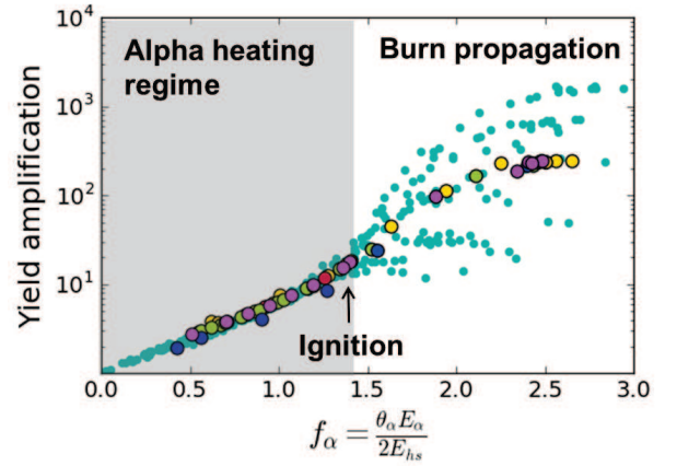
FIG. 1: The yield amplification is plotted as a function of f_\alpha for the ensemble of 1-D LILAC [14] simulations (turquoise points). In the alpha-heating regime ( f_\alpha < 1.4 ), the yield amplification depends uniquely on f_\alpha regardless of the target mass, areal density, and temperature. After f_\alpha = 1.4 , shell mass and burnup fraction determine the maximum fusion yield. The yellow, red, green, and dark blue points respectively represent 2-D DRACO [15] single mode simulations of modes 2, 4, 6, and 10. The purple points are multi-mode simulations perturbed by modes 2 and 4.
