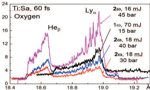
Figure 1. Plasma emission spectra in the spectral range of 18.5–19.2 Å at different experimental conditions. The contour of the O VIII Ly \alpha has characteristic intensity modulations in the blue wing of line that are especially conspicuous when the clusters are heated the 2 \omega . Laser parameters: \tau = 60 fs, E_{1\omega} \sim 70 mJ, E_{2\omega} \sim 20 mJ [1]
