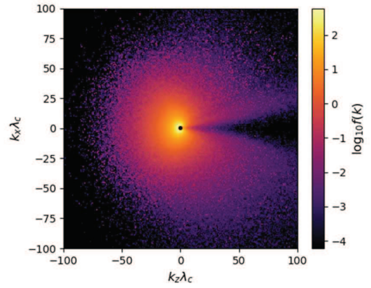
Figure 2. Momentum (wavenumber) distribution of the gamma rays.
