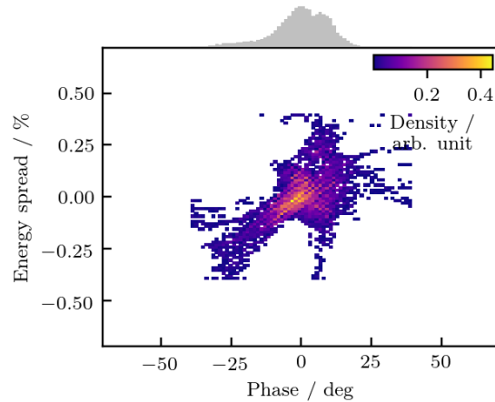
Figure 5: Reconstructed phase space with the NNLS solver (108 MHz).
