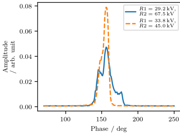
Figure 3: Bunch shape samples for two different rebuncher settings measured with the BSM (108 MHz).
