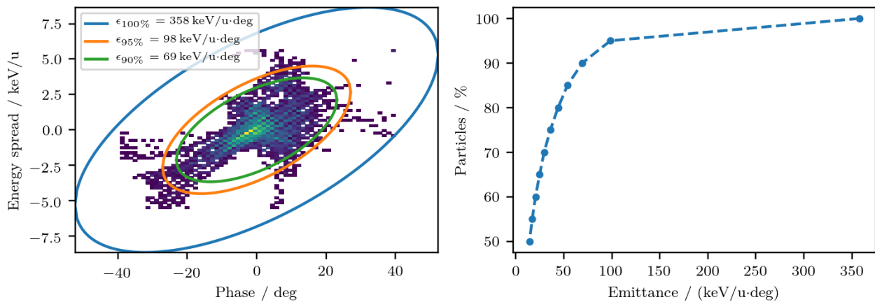
Figure 6: Brilliance analysis of the reconstructed distribution. Samples of the fitted ellipses around a fraction of the density distribution (left) and relation of the emittance on the fraction of particles (right).
