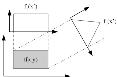
Figure 2: Example of reconstruction setup for a linear transformation between image and histogram. The observed histograms f_i(x') constrain the shape of the reconstructed object [31].
