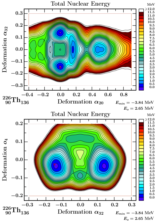
Fig. 1. Top: Total energy surfaces for ^{226}\text{Th} showing the presence of tetrahedral symmetry minima at \alpha_{20} = 0 in competition with quadrupole symmetry minima. At each point, the energy was minimised over octahedral symmetry deformations o_4 and o_6 , cf. Eqs. (7) and (8). Bottom: Projection over t_3 -tetrahedral vs. o_4 -octahedral symmetry deformations minimised over o_6 showing combined tetrahedral-octahedral symmetry minima at o_4 \approx -0.04 . By convention we normalise the macroscopic energy to zero at zero deformation; E_o is the corresponding shell-energy, whereas E_{\min} denotes the energy at the absolute minimum.
