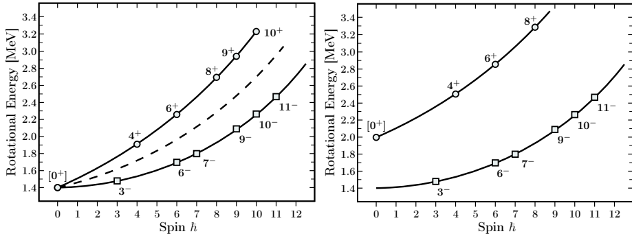
Fig. 2. Qualitative. Left: The characteristic configuration of two parabolic energy vs. spin sequences of opposite parities aiming at a common I^\pi = 0^+ lowest energy point (tetrahedral symmetry ‘ground-state’). In the case of pure tetrahedral symmetry, the two branches are expected to form a single one coinciding with the dashed line (for details cf. Ref. [10]). Right: Hypothetical pure octahedral symmetry configuration. The two auxiliary curves are expected to be approximately parallel and they are not expected to join the common I^\pi = 0^+ point at the bottom. This feature can be used to distinguish between the scenarios of single or coexisting symmetry configurations.
