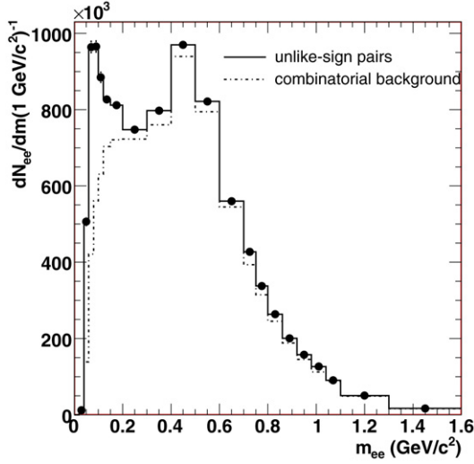
Fig. 1. Unlike-sign pair yield (histogram) and combinatorial background (dashed curve). See text for explanation.
