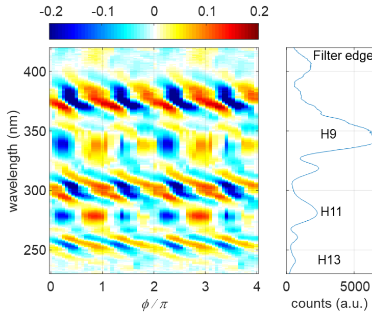
Fig. 5. CEP dependence of the high harmonic spectrum generated by a few-cycle laser pulses at 3.1 \mu\text{m} . The color code denotes the normalized difference between the signal obtained at a given CEP and the CEP-averaged signal. The relative CEP \phi is obtained from the interference fringes between the harmonics using the method described in the text. Harmonic orders and the filter edge near 400 nm are indicated in the spectrum
