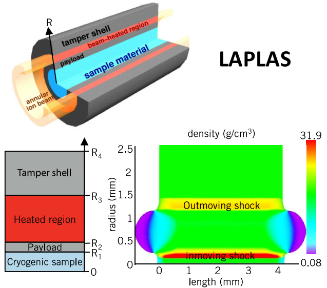
FIG. 4. The LAPLAS scheme uses annular heavy ion beams ( U^{28+} ) to heat a material driver inside a cylindrical tamper shell. Subsequent material heating drives a cylindrical compression of the sample material. Relatively uniform HED matter can be formed and probed with this technique up to Mbar pressures. The example shown above 70 is a simulation of an iron sample compressed by a tungsten shell up to a density of 18 g/cm 3 , temperature of 1260 K, and pressure of 7.6 Mbar using a 1.5-GeV/u uranium beam from the SIS-100 with a 75 ns bunch of 5 \times 10^{11} ions.
