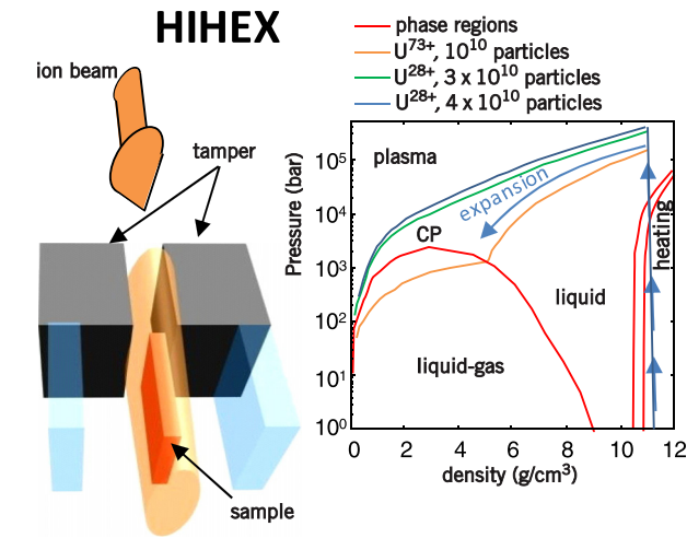
FIG. 3. The HIHEX scheme where ion beams ( U^{28+} or U^{73+} ) heat a material sample confined between two tampers. The sample heats isochorically with subsequent isentropic expansion. Using the SIS-100 parameters envisaged for FAIR Day-one experiments, the HIHEX scheme will be able to fully explore the critical points of many periodic system metals. Right-hand side: HIHEX predictions for lead for various ion-beam intensities. 54
