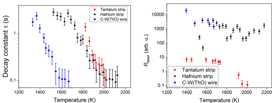
Fig. 3 Left: Decay constant (desorption time) as a function of the filament temperature. Right: Ratio of laser photo ions to surface ions as function of the filament temperature
