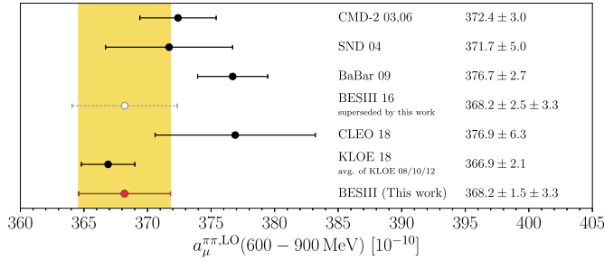
Fig. 3. Comparison of the updated calculation of the leading-order (LO) hadronic vacuum polarization contribution to (g-2)_\mu due to \pi^+\pi^- in the energy range 600 - 900 MeV from BESIII and the corresponding results from CMD-2 [13,14], SND [15], BaBar [11], BESIII 16 [1], CLEO [16], and KLOE [17]. The respective values are taken from the white paper of the Muon g-2 Theory Initiative [2,3,18–22]. The yellow band indicates the 1\sigma range of the updated BESIII result.
