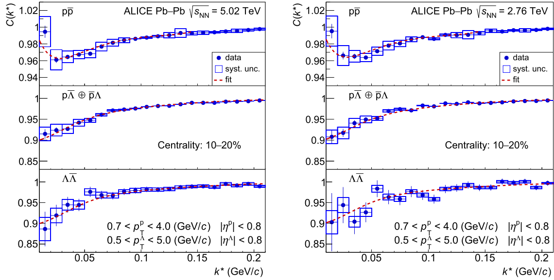
Fig. 3. Correlation functions of p\bar{p} , p\bar{\Lambda} \oplus p\bar{\Lambda} , and \Lambda\bar{\Lambda} pairs for Pb-Pb collisions at \sqrt{s_{NN}} = 5.02 TeV (left) and \sqrt{s_{NN}} = 2.76 TeV (right) together with the simultaneous femtoscopic fit for the 10–20% centrality class.
