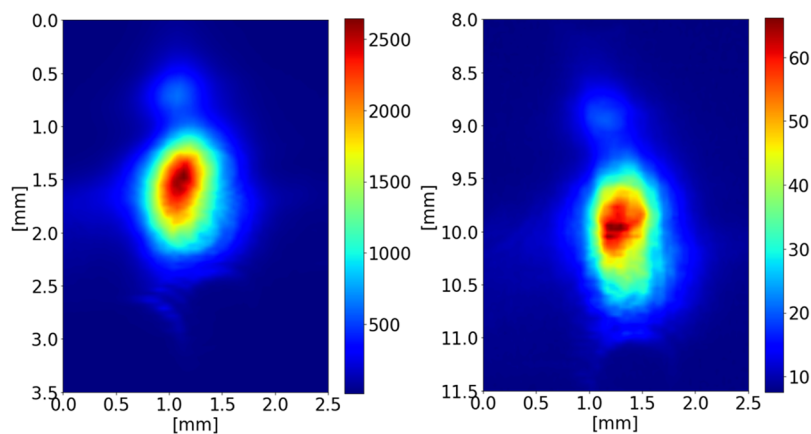
FIG. 2. A comparison of the beam profiles 80 m after the monochromators on a YAG-screen. On the left side is displayed the beam after two reflections from the highly polished Si (111) crystals. The right side shows the beam after the additional Si (533) monochromator without high quality polishing. Both images show the average over roughly 1800 shots of the FEL. This demonstrates that the spatial profile of the coherent FEL beam is preserved by the Si (533) channel-cut monochromator.
