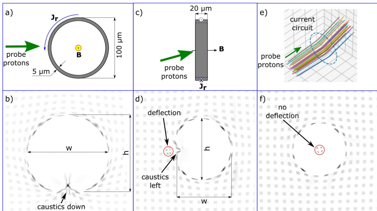
Figure 3. Proton radiographs on the example of the ring current circuit. a), c) – illustration of two probing geometries – perpendicular to the target axis and almost parallel to it respectively; b), d) – corresponding simulated radiographs; e) illustration of deflection for protons passing through the target centre; f) simulated radiograph for quasi-parallel probing geometry.
