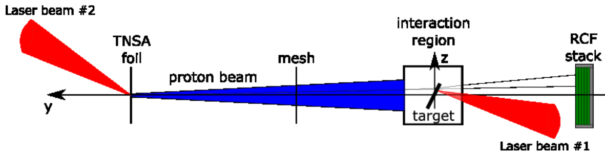
Figure 1. Principal scheme of proton radiography.
