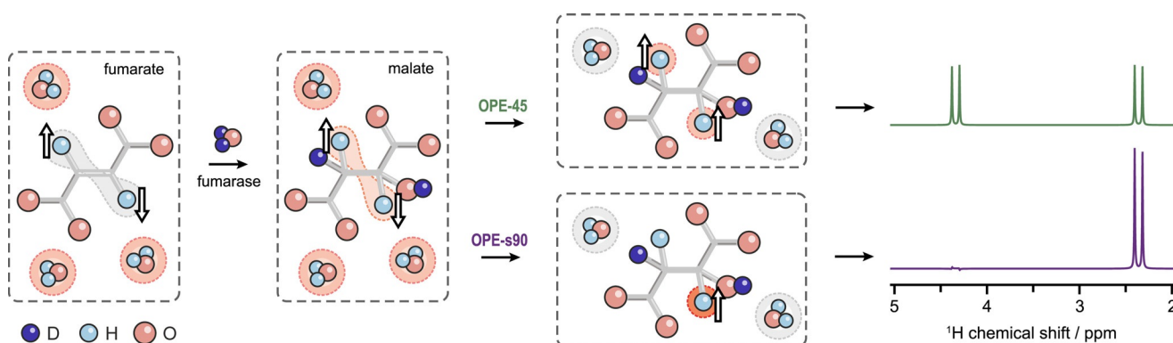
Figure 2. A graphical depiction of hyperpolarized fumarate being converted into malate- D_2 , followed by the application of OPE-45 or OPE-s90 to convert the antiphase proton spin order into in-phase magnetization, and suppress background signals from water. The white arrows represent different types of spin order, with up-down arrows in the first two frames indicating the absence of net magnetization on the proton spins. Red and grey shading is used to represent observable and unobservable spin groups, respectively, from different species throughout the experiment. Simulations of the resulting hyperpolarized spectra are shown on the right, using the NMR parameters given in Figure 1. Note that in principle OPE-45 and OPE-s90 produce the same integral of the proton signal.
