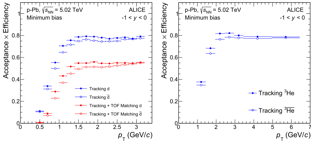
Fig. 2. Tracking acceptance \times efficiency correction for (anti-)deuterons (left) and for {}^3\text{He} and \bar{{}^3\text{He}} (right) in the minimum-bias class. The efficiencies for anti-nuclei are lower due to the larger cross-section for hadronic interactions.
