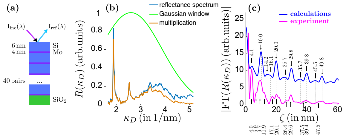
Fig. 4 Schematic of the Mo/Si multilayer structure studied using “water-window” XCT (a). The sample consists of 40 pairs of 6 nm-thick silicon and 4 nm-thick molybdenum layers deposited on a SiO 2 substrate. b The measured reflectivity (teal line) is filtered with a Gaussian-type window function (green) to suppress the Fourier arti-
