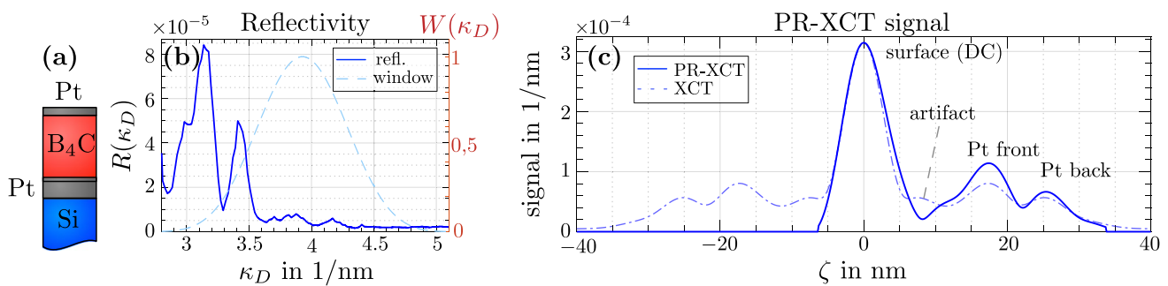
Fig. 3 Results of an XCT investigation in the water transmission window: sample (a) consists of a 8 nm-thick Pt layer buried under 18 nm of boron carbide B_4C . b Recorded reflected spectral intensity in the water window 280–530 eV (4.4–2.3 nm) of the layer system. The solid line (blue) represents the interpolation of data acquired for different monochromator positions. The dashed curve (light blue) is the Kaiser–Bessel spectral window used to suppress Fourier artifacts. c Reconstructed depth profile (dot–dashed line) by Fourier transform of experimentally measured reflectivity. The frontside and backside of
